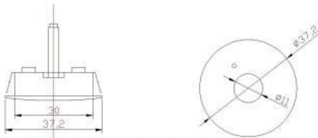
Load(Spotlight)mechanical Outline(unit:mm)
