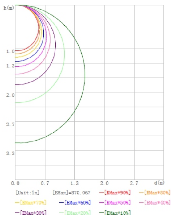
C0 Space ISO Illuminance Curve
